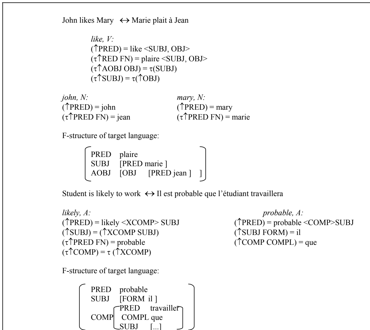
Fig.2: Constraint-based formalism (LFG)
