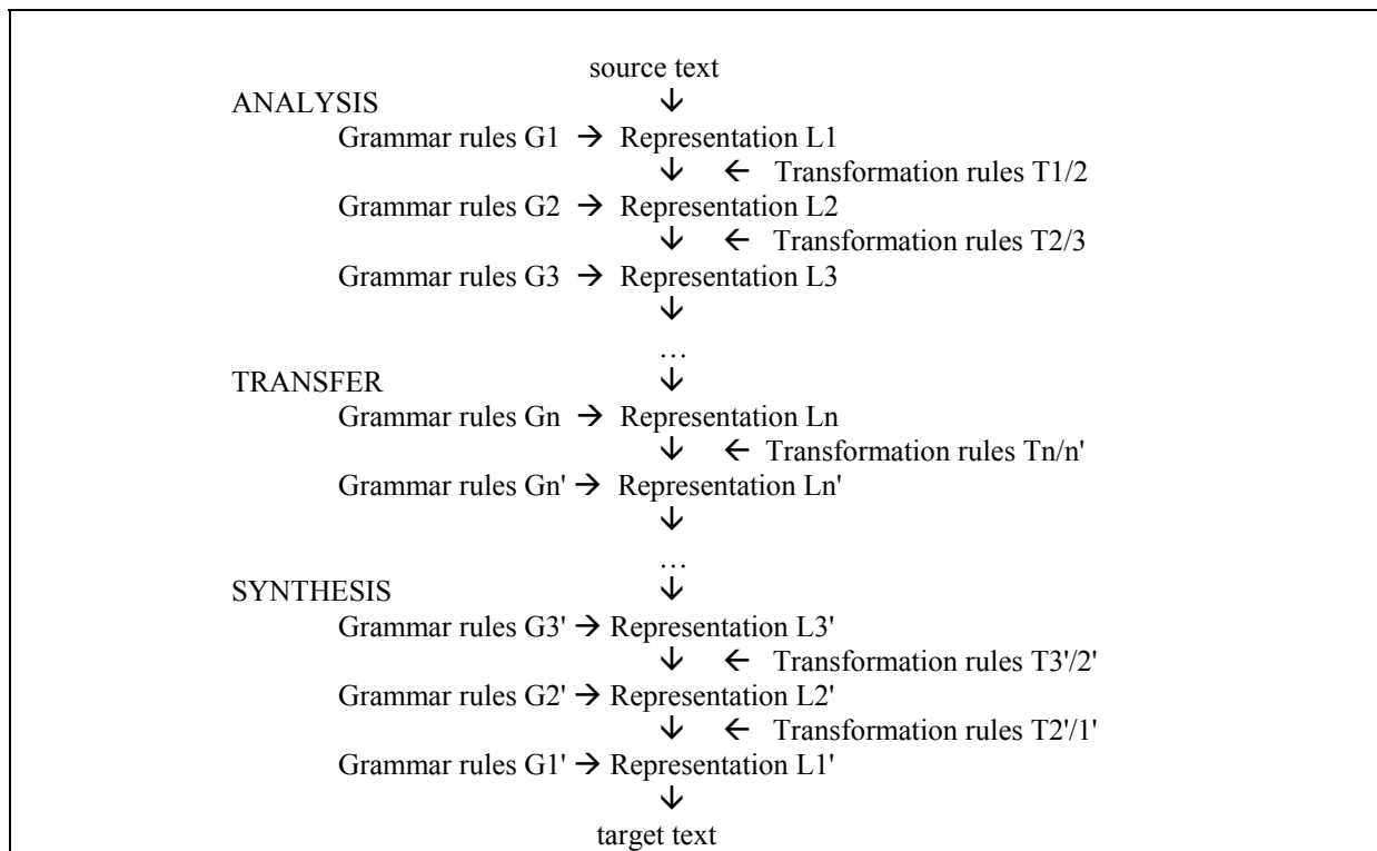
Figure 1: Rules of formation and transformation (Eurotra)
